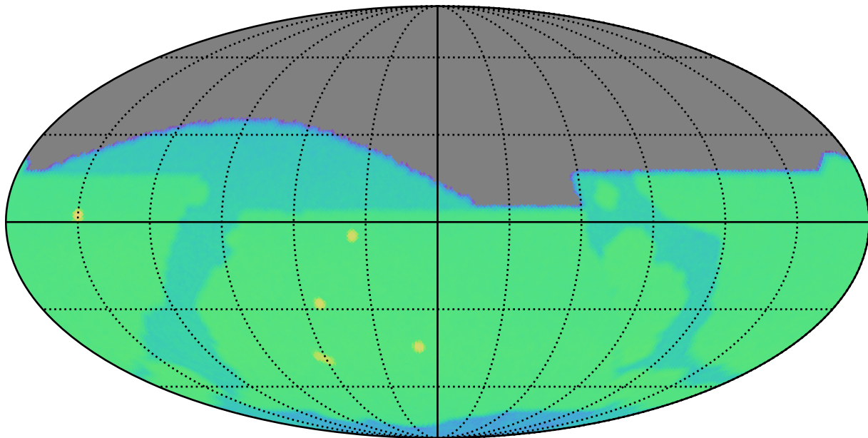
noroll_mjdp365_v3.4_10yrs r: SurfaceBrightLimit
