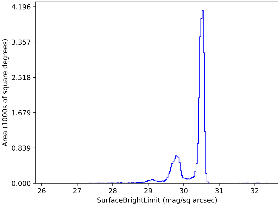
noroll_mjdp365_v3.4_10yrs r: SurfaceBrightLimit
