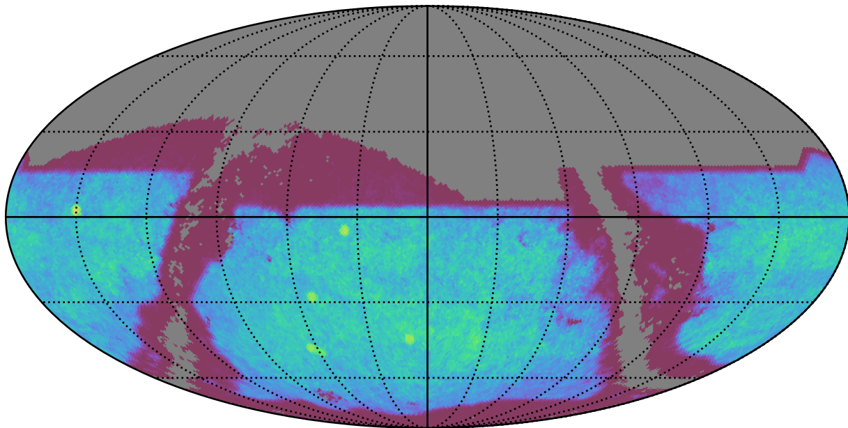
noroll_mjdp365_v3.4_10yrs : SNSLMetric
