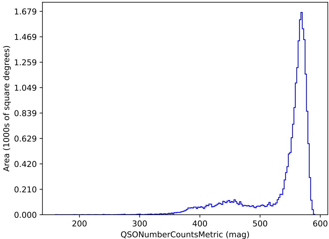
noroll_mjdp365_v3.4_10yrs y band and non-DD: QSONumberCountsMetric
