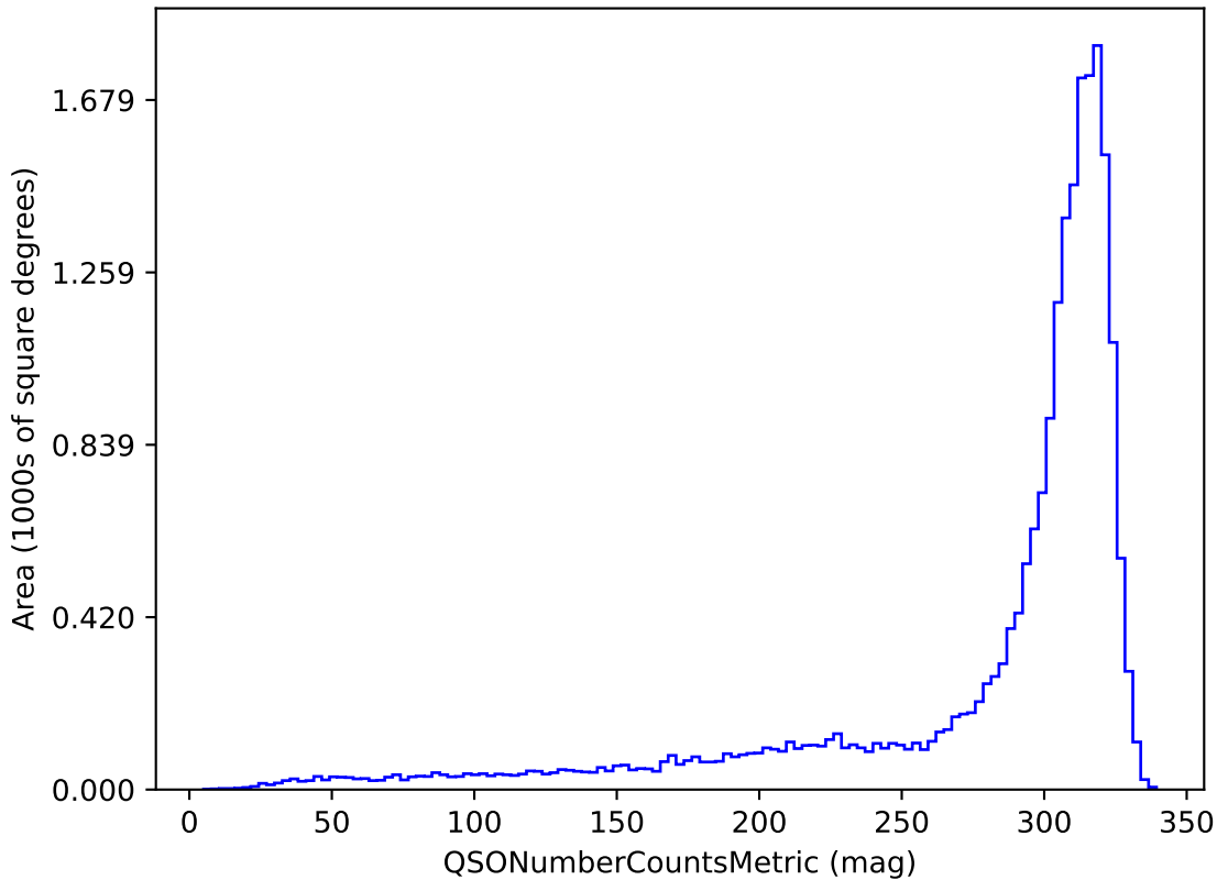
noroll_mjdp365_v3.4_10yrs u band and non-DD: QSONumberCountsMetric
