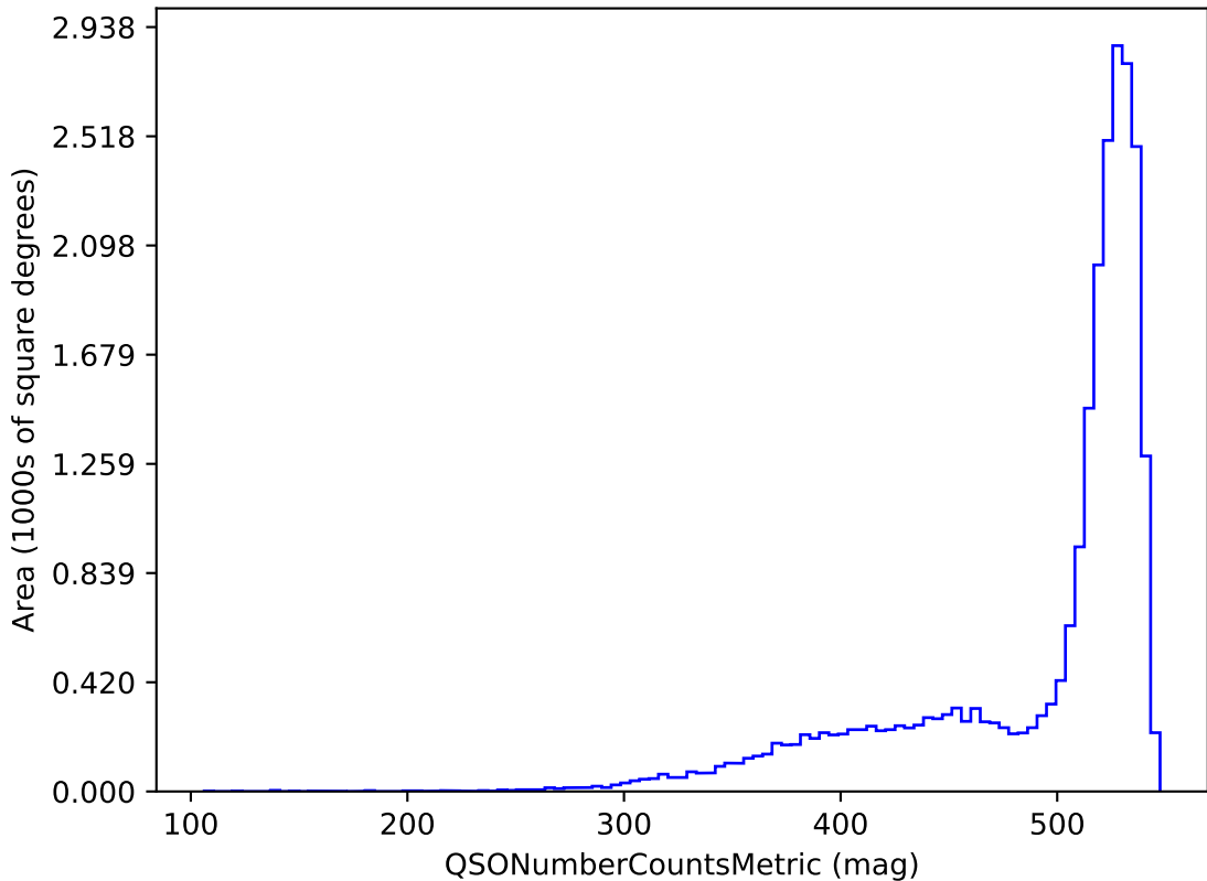
noroll_mjdp365_v3.4_10yrs r band and non-DD: QSONumberCountsMetric
