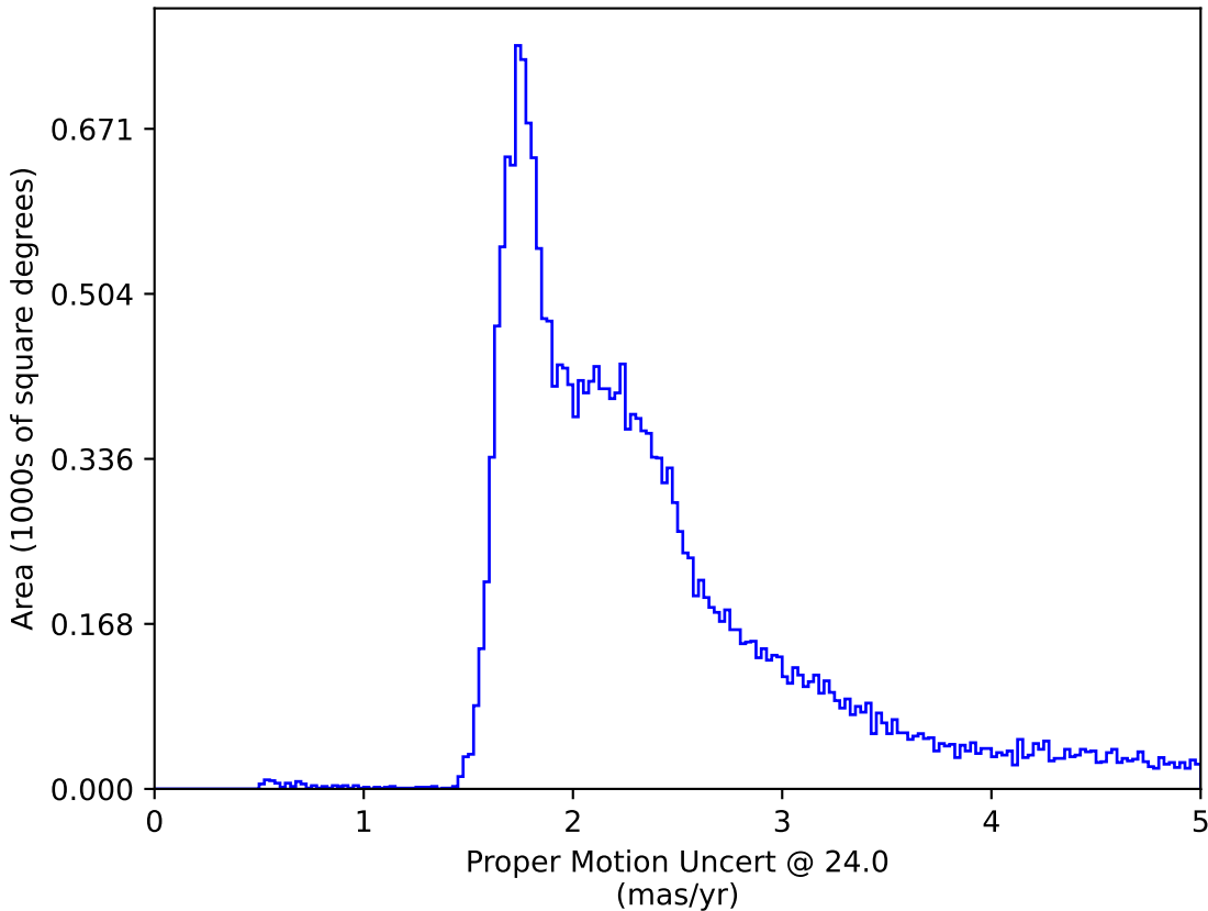
noroll_mjdp365_v3.4_10yrs : Proper Motion Uncert @ 24.0
