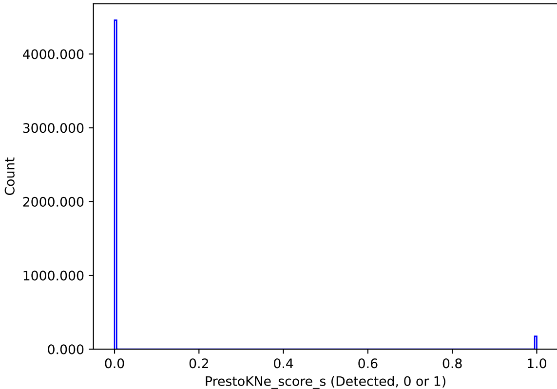
noroll_mjdp365_v3.4_10yrs : PrestoKNe_score_s
