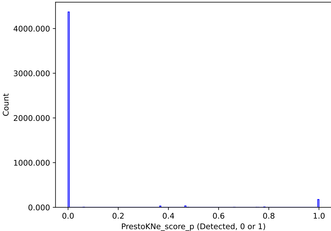
noroll_mjdp365_v3.4_10yrs : PrestoKNe_score_p
