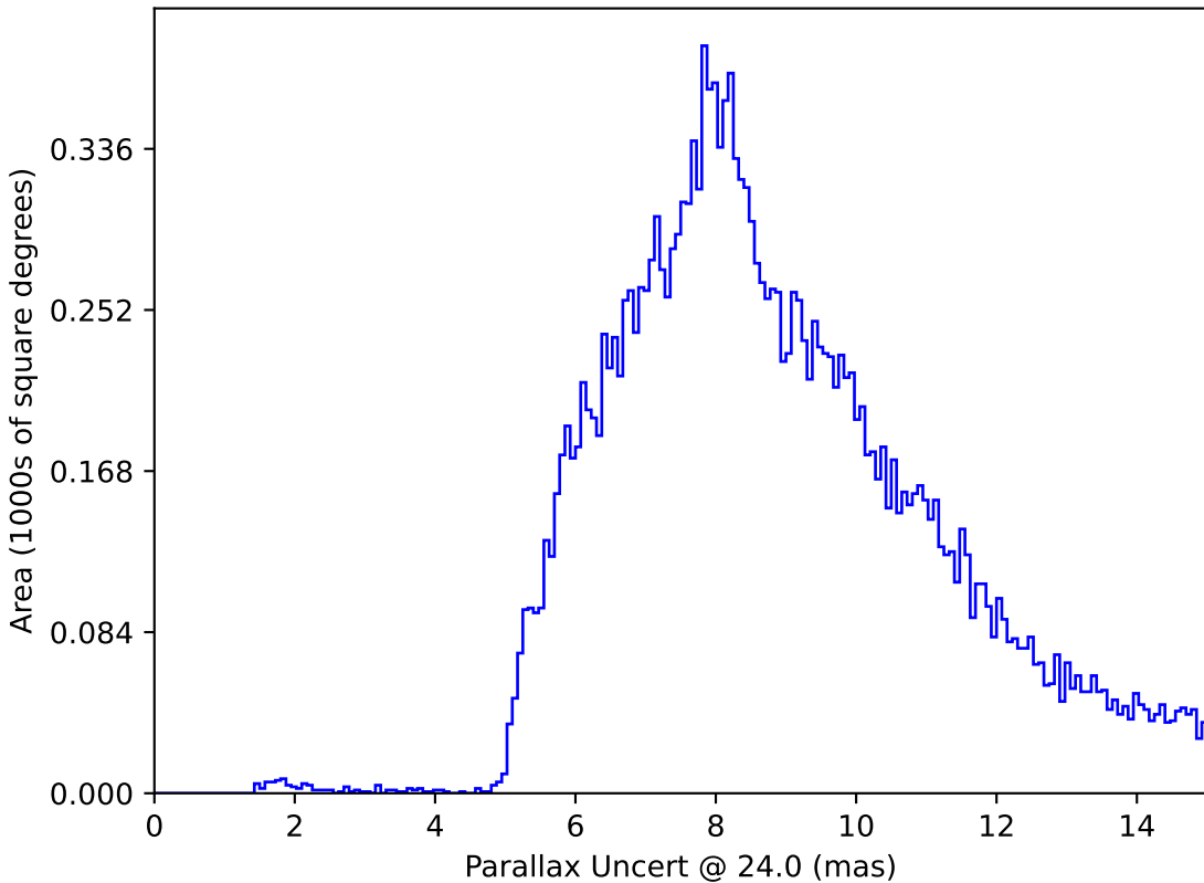
noroll_mjdp365_v3.4_10yrs : Parallax Uncert @ 24.0
