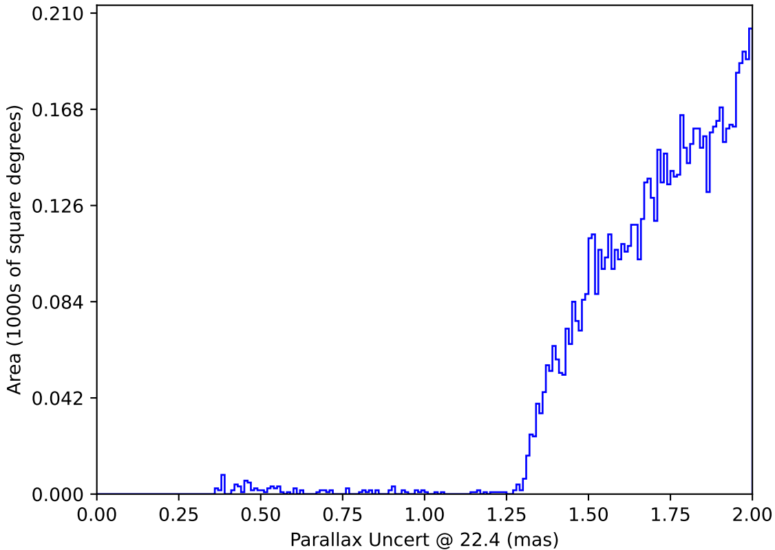
noroll_mjdp365_v3.4_10yrs : Parallax Uncert @ 22.4
