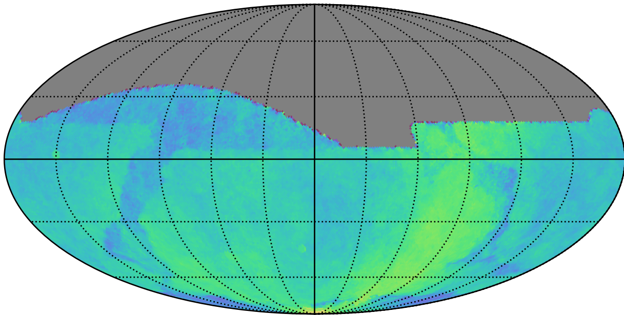
noroll_mjdp365_v3.4_10yrs : Parallax Coverage @ 24.0
