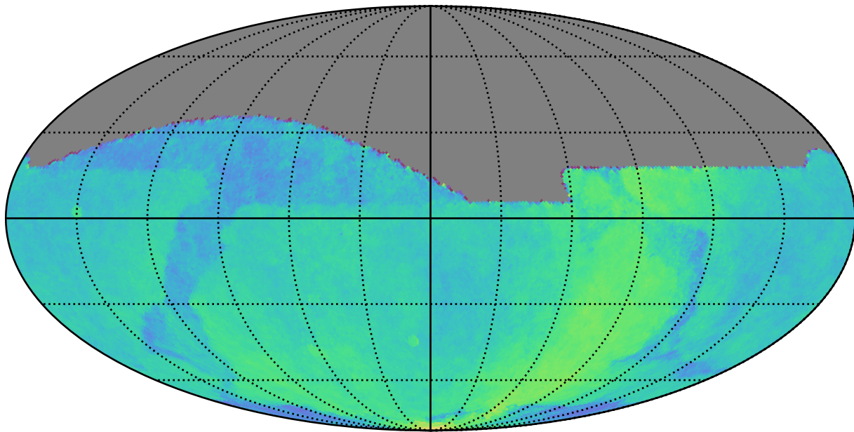
noroll_mjdp365_v3.4_10yrs : Parallax Coverage @ 22.4
