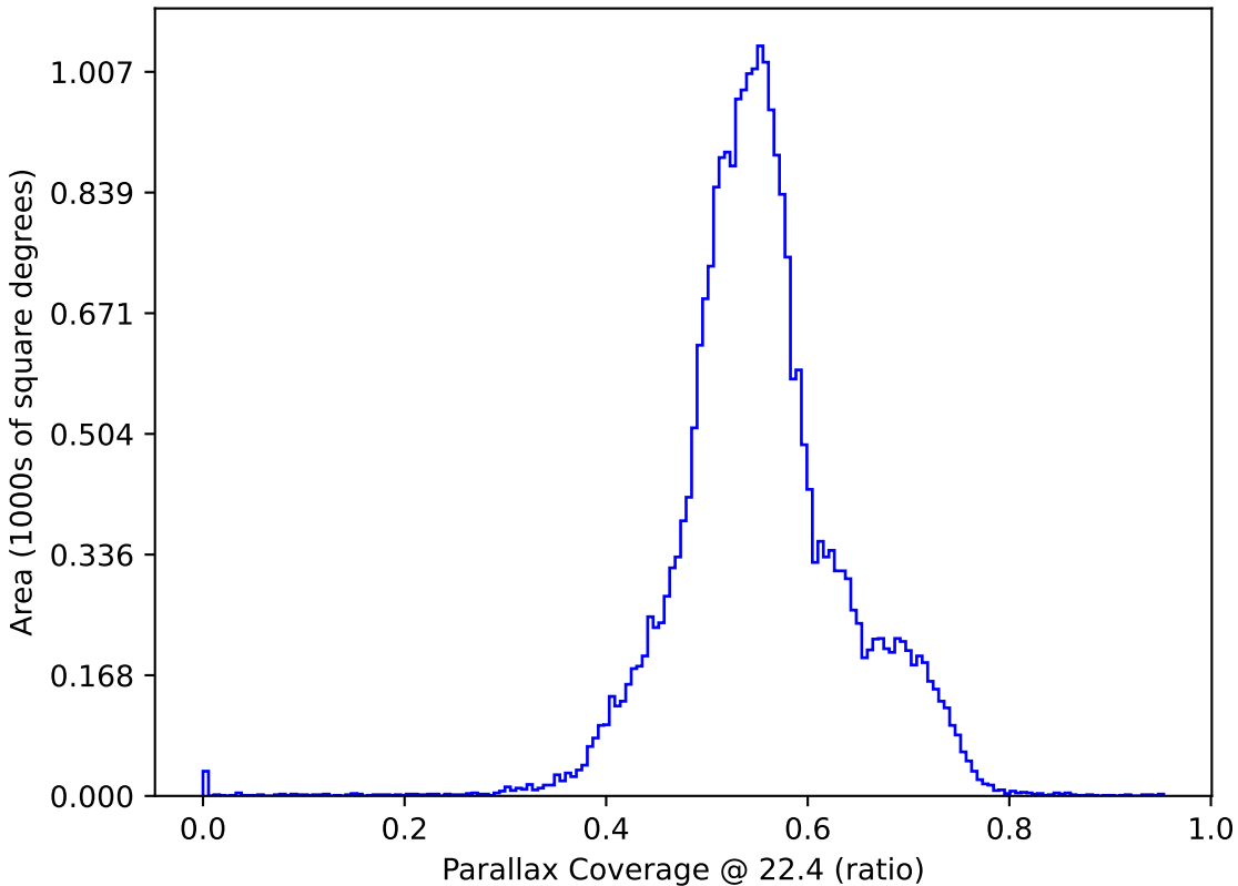
noroll_mjdp365_v3.4_10yrs : Parallax Coverage @ 22.4
