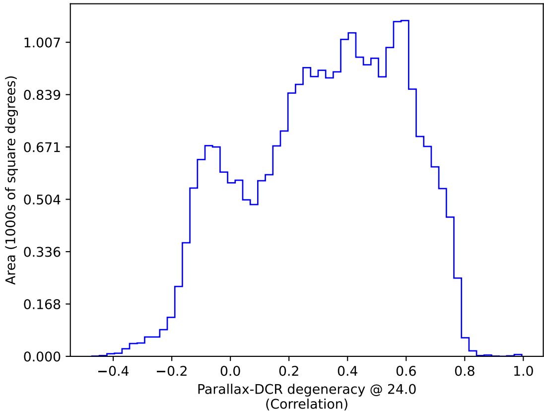
noroll_mjdp365_v3.4_10yrs : Parallax-DCR degeneracy @ 24.0
