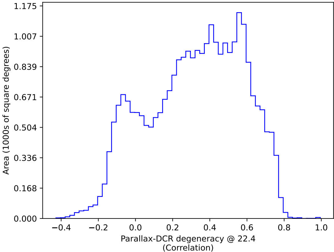
noroll_mjdp365_v3.4_10yrs : Parallax-DCR degeneracy @ 22.4
