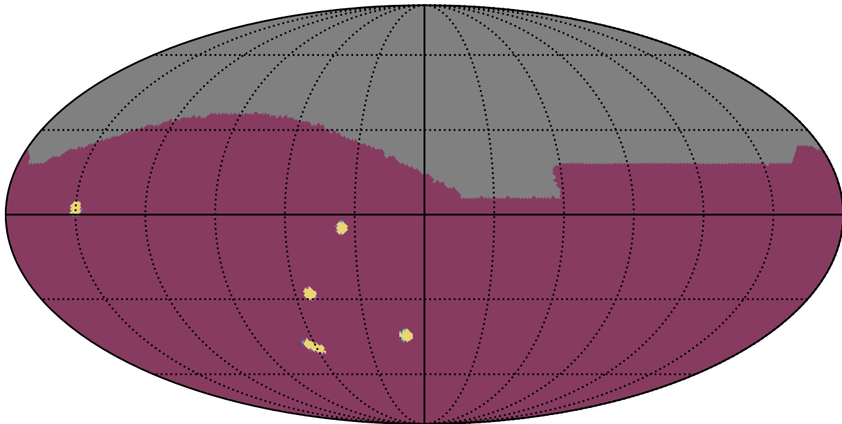
noroll_mjdp365_v3.4_10yrs : NumberOfQuickRevisits
