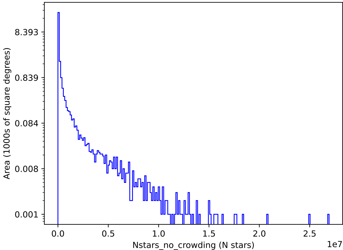
noroll_mjdp365_v3.4_10yrs z: Nstars_no_crowding
