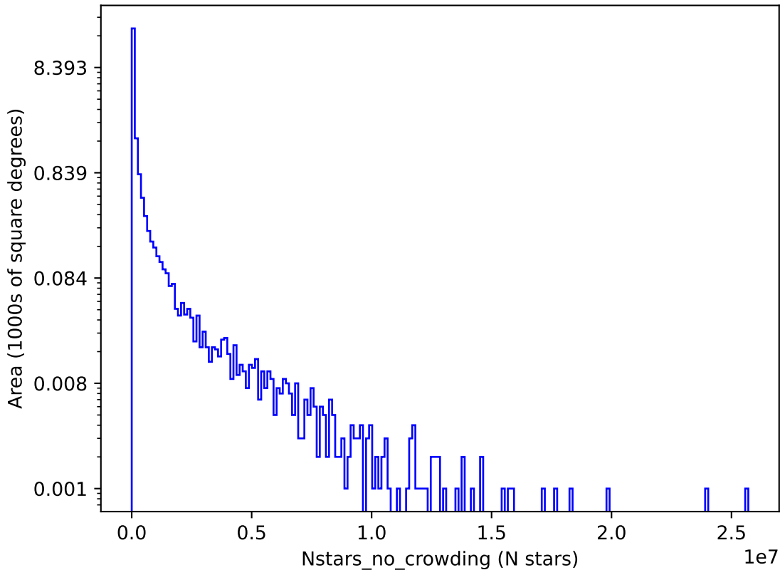
noroll_mjdp365_v3.4_10yrs y: Nstars_no_crowding
