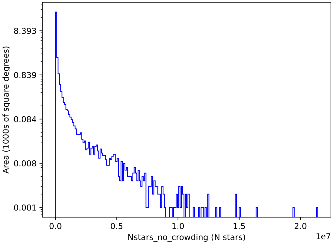
noroll_mjdp365_v3.4_10yrs r: Nstars_no_crowding
