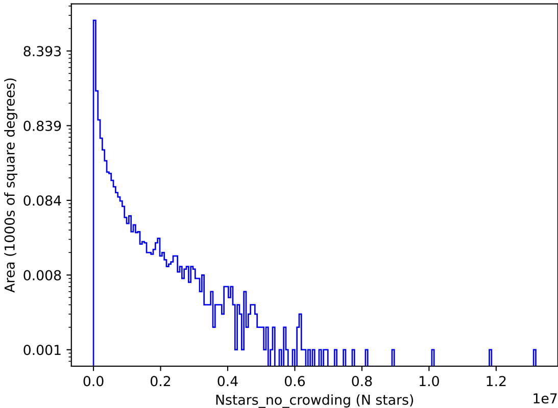
noroll_mjdp365_v3.4_10yrs g: Nstars_no_crowding
