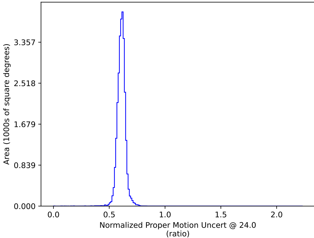
noroll_mjdp365_v3.4_10yrs : Normalized Proper Motion Uncert @ 24.0
