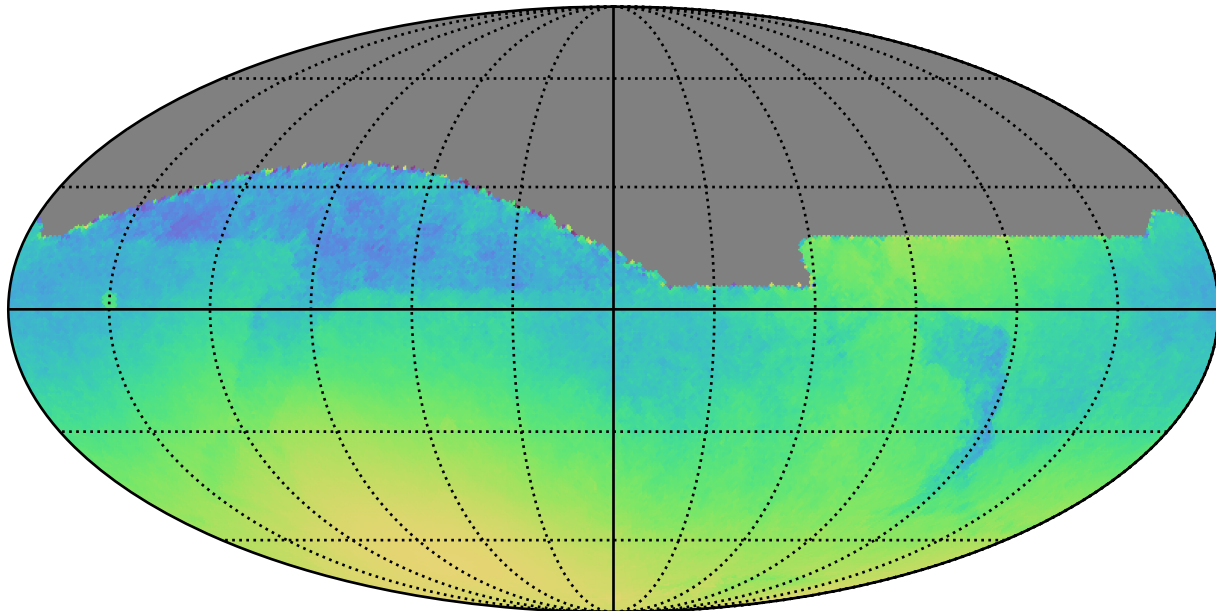
noroll_mjdp365_v3.4_10yrs : Normalized Parallax Uncert @ 24.0
