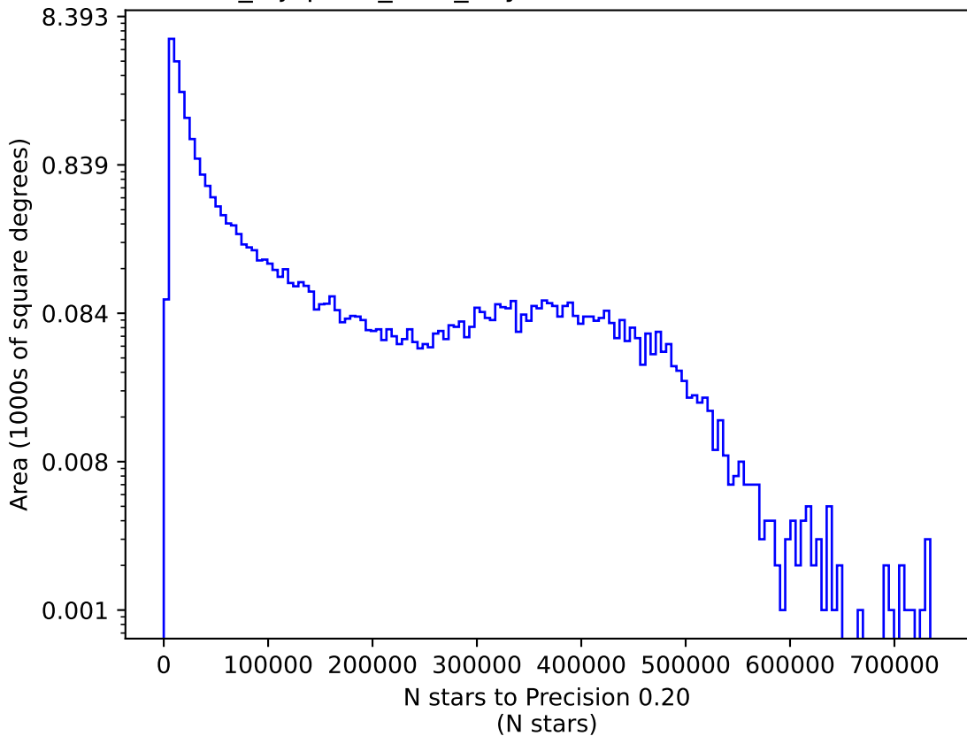
noroll_mjdp365_v3.4_10yrs z: N stars to Precision 0.20
