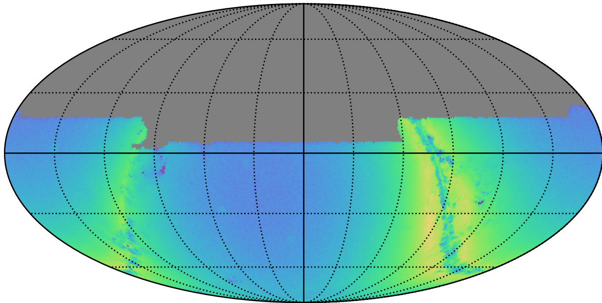
noroll_mjdp365_v3.4_10yrs u: N stars to Precision 0.20
