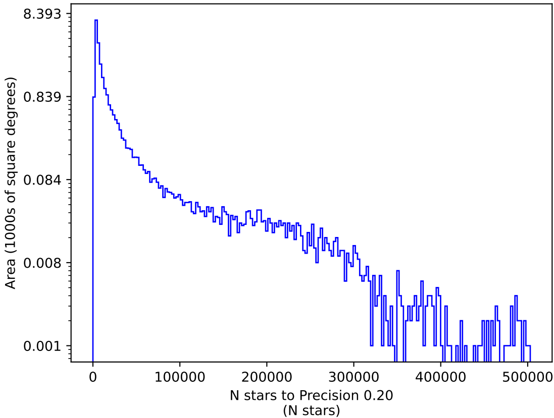
noroll_mjdp365_v3.4_10yrs u: N stars to Precision 0.20
