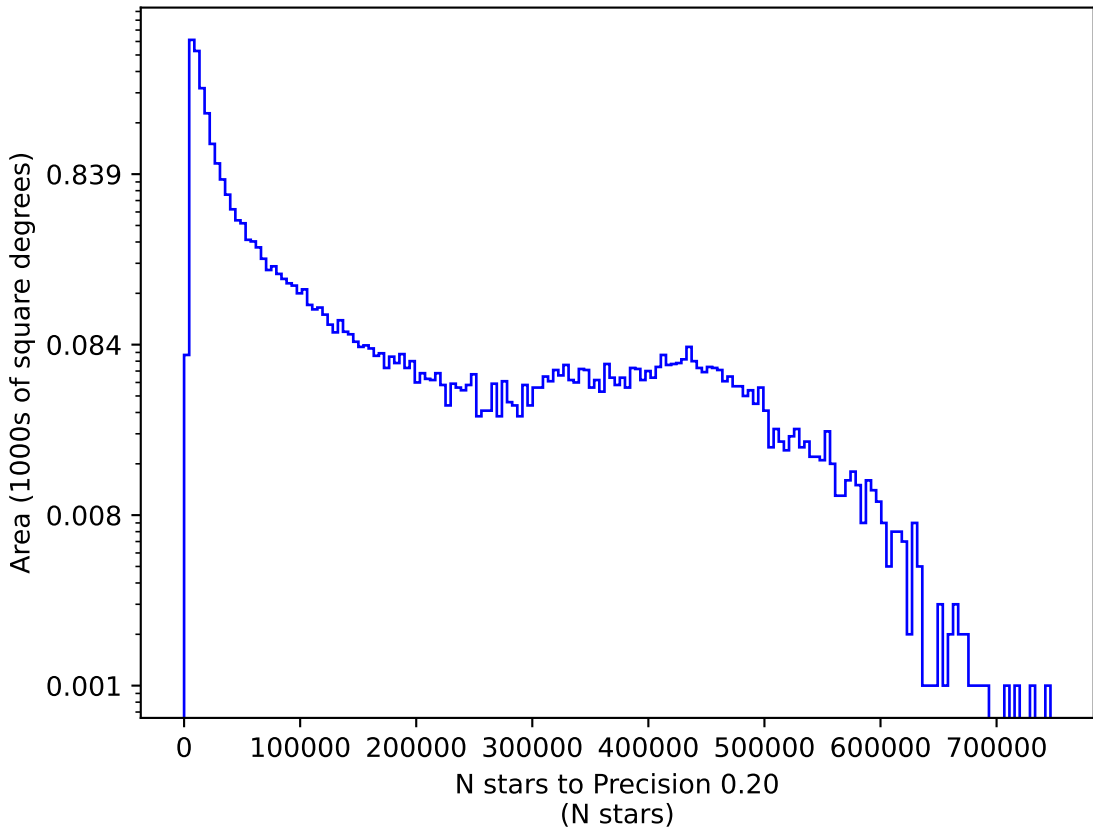
noroll_mjdp365_v3.4_10yrs r: N stars to Precision 0.20
