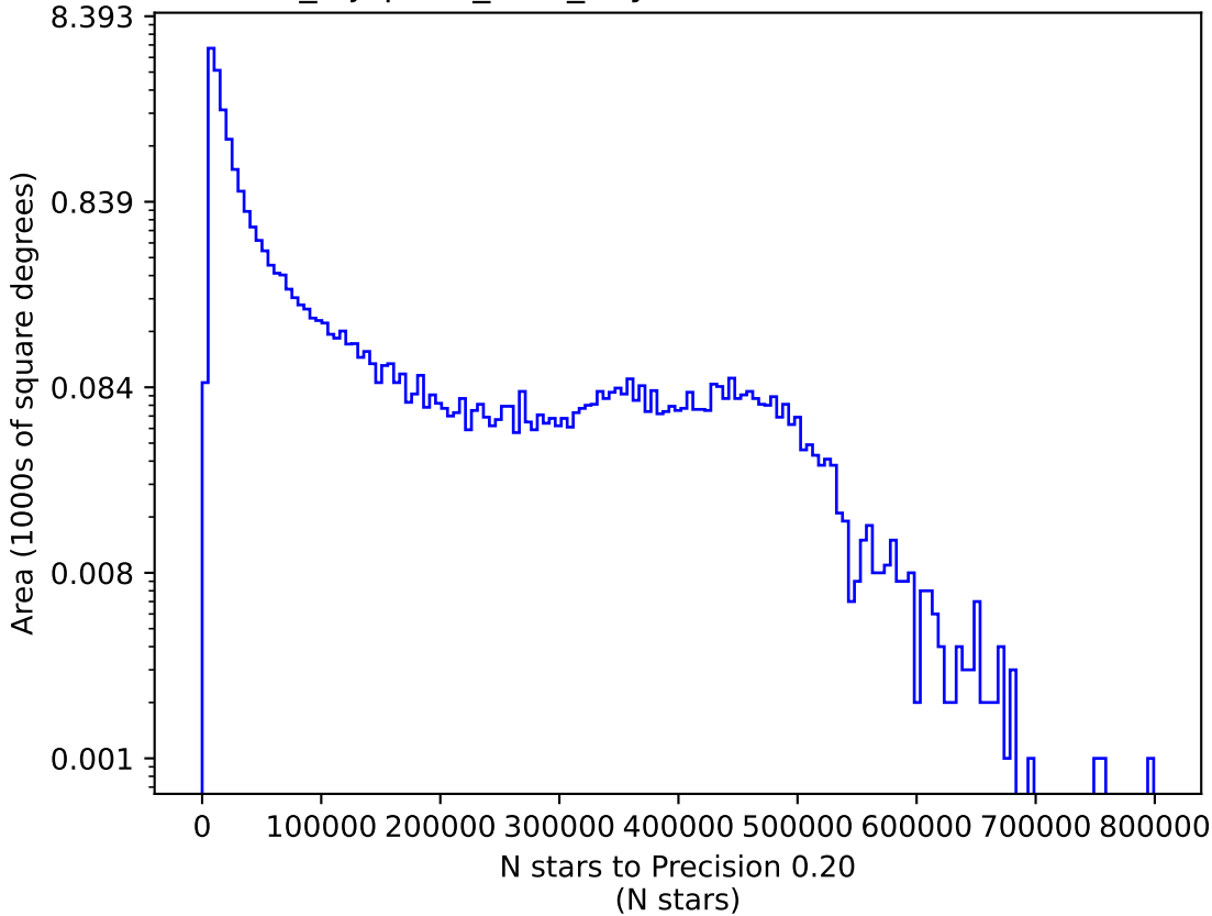
noroll_mjdp365_v3.4_10yrs i: N stars to Precision 0.20
