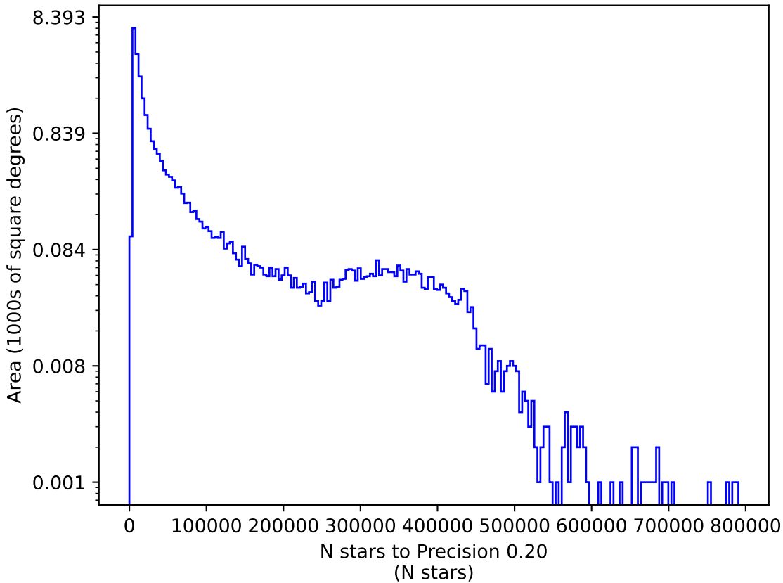
noroll_mjdp365_v3.4_10yrs g: N stars to Precision 0.20
