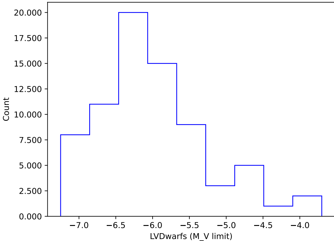
noroll_mjdp365_v3.4_10yrs gi: LVDwarfs
