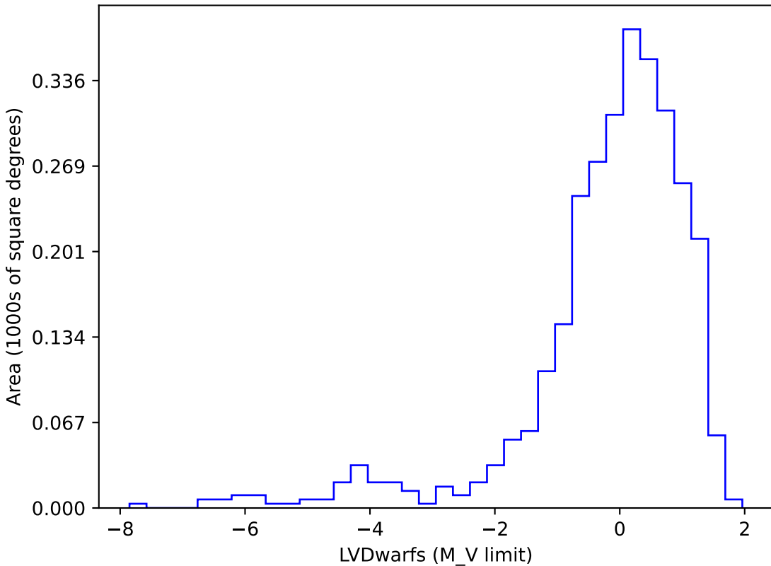
noroll_mjdp365_v3.4_10yrs gi SCP: LVDwarfs
