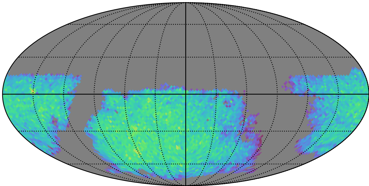
noroll_mjdp365_v3.4_10yrs gi: LVDwarfs
