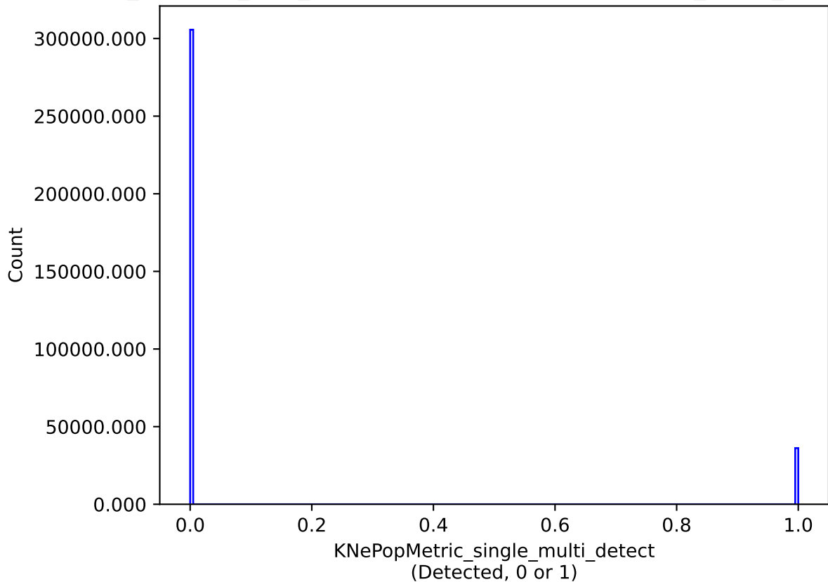
noroll_mjdp365_v3.4_10yrs single model: KNePopMetric_single_multi_detect
