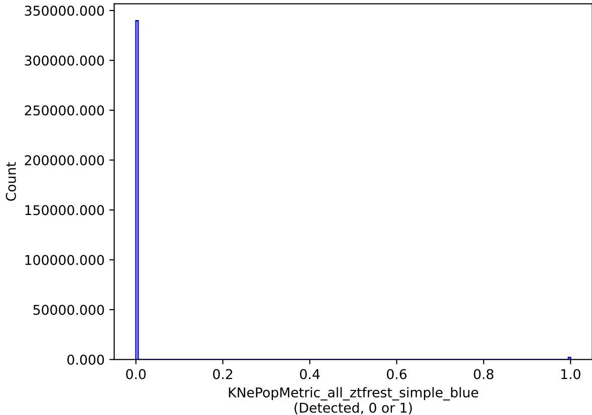
noroll_mjdp365_v3.4_10yrs all models: KNePopMetric_all_ztfrest_simple_blue
