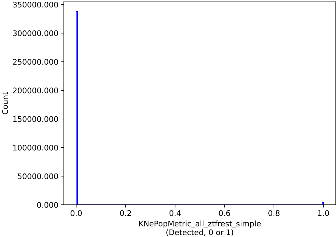
noroll_mjdp365_v3.4_10yrs all models: KNePopMetric_all_ztfrest_simple
