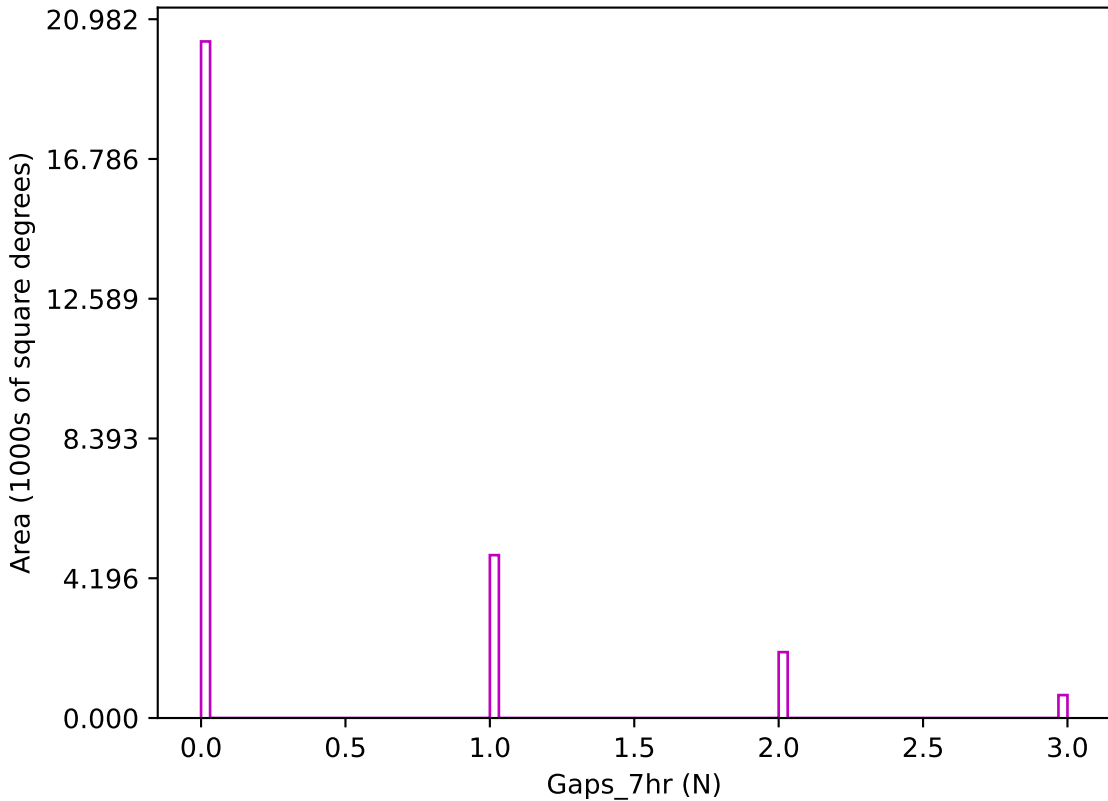
noroll_mjdp365_v3.4_10yrs z band: Gaps_7hr
