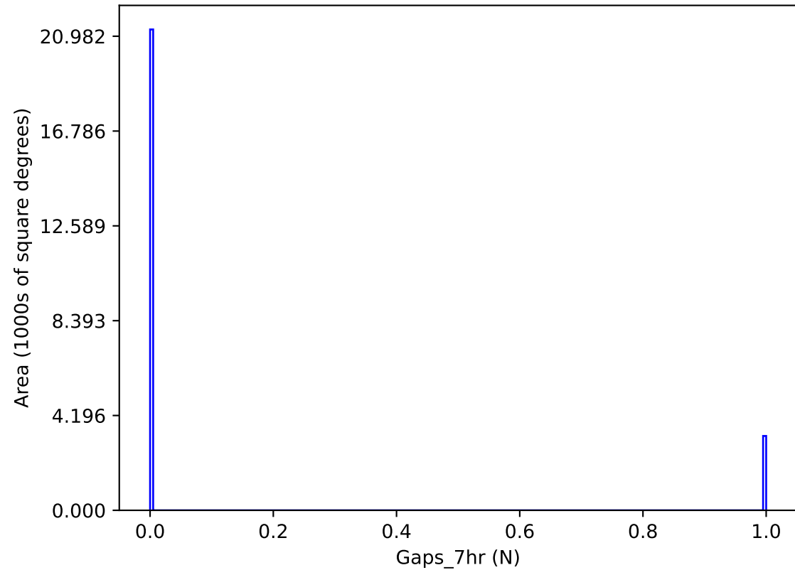
noroll_mjdp365_v3.4_10yrs y band: Gaps_7hr
