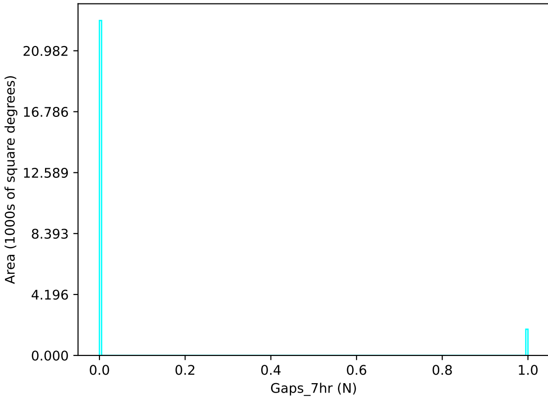
noroll_mjdp365_v3.4_10yrs u band: Gaps_7hr
