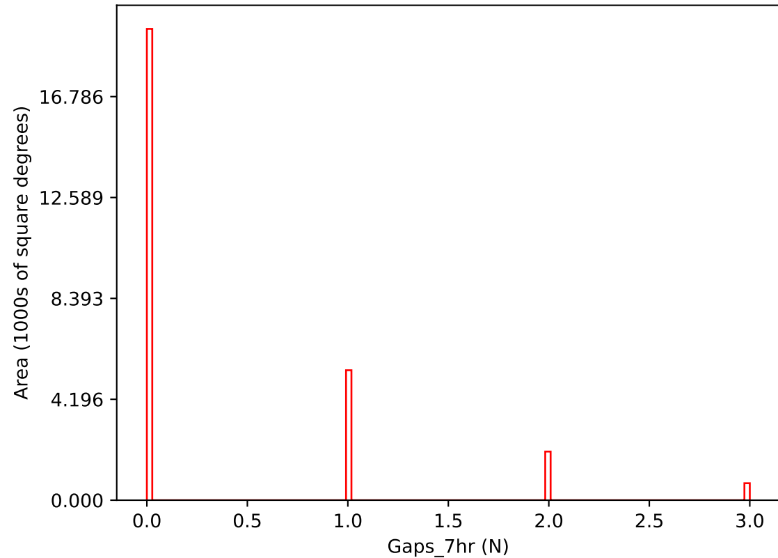
noroll_mjdp365_v3.4_10yrs i band: Gaps_7hr
