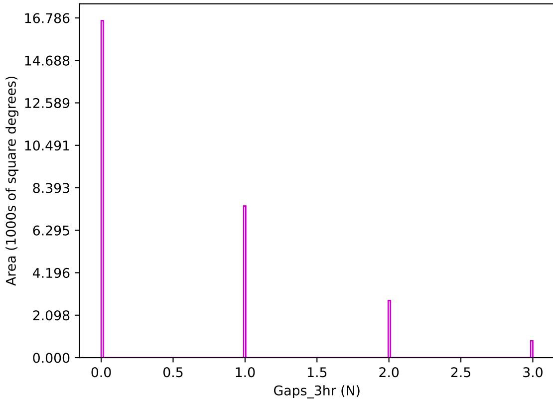
noroll_mjdp365_v3.4_10yrs z band: Gaps_3hr
