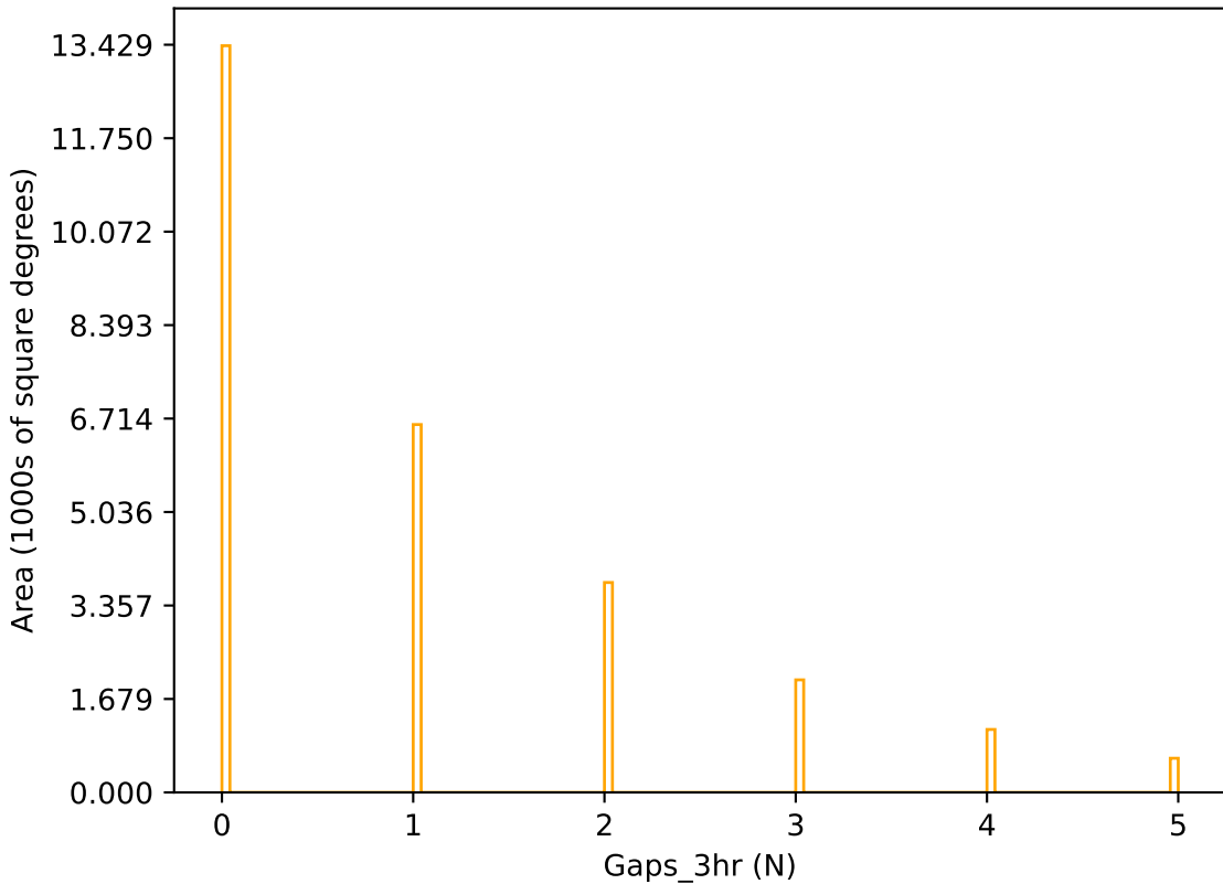
noroll_mjdp365_v3.4_10yrs r band: Gaps_3hr
