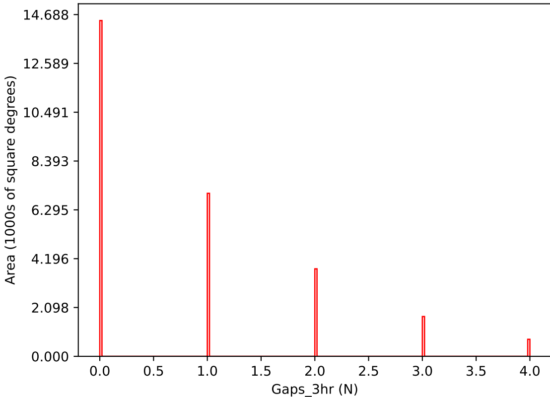
noroll_mjdp365_v3.4_10yrs i band: Gaps_3hr
