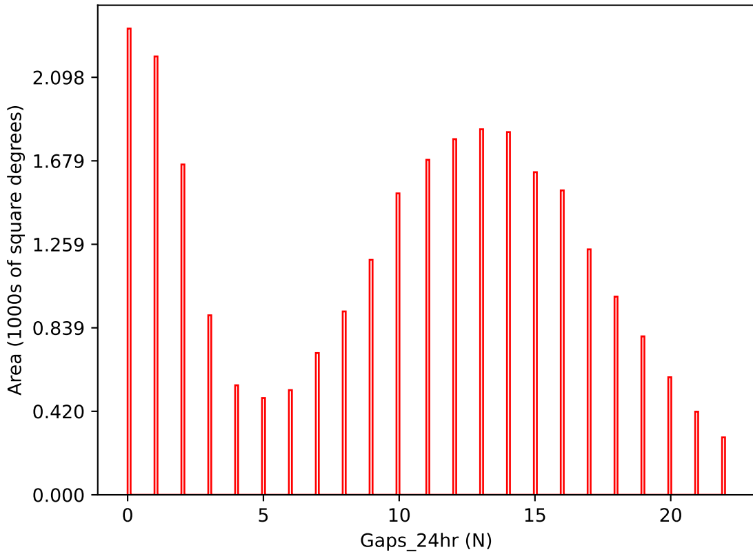
noroll_mjdp365_v3.4_10yrs i band: Gaps_24hr
