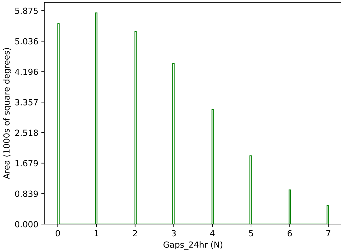
noroll_mjdp365_v3.4_10yrs g band: Gaps_24hr
