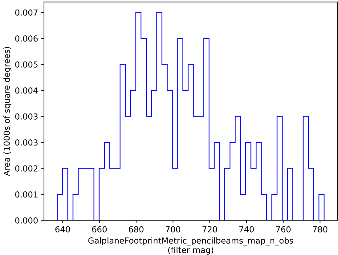
noroll_mjdp365_v3.4_10yrs : GalplaneFootprintMetric_pencilbeams_map_n_obs
