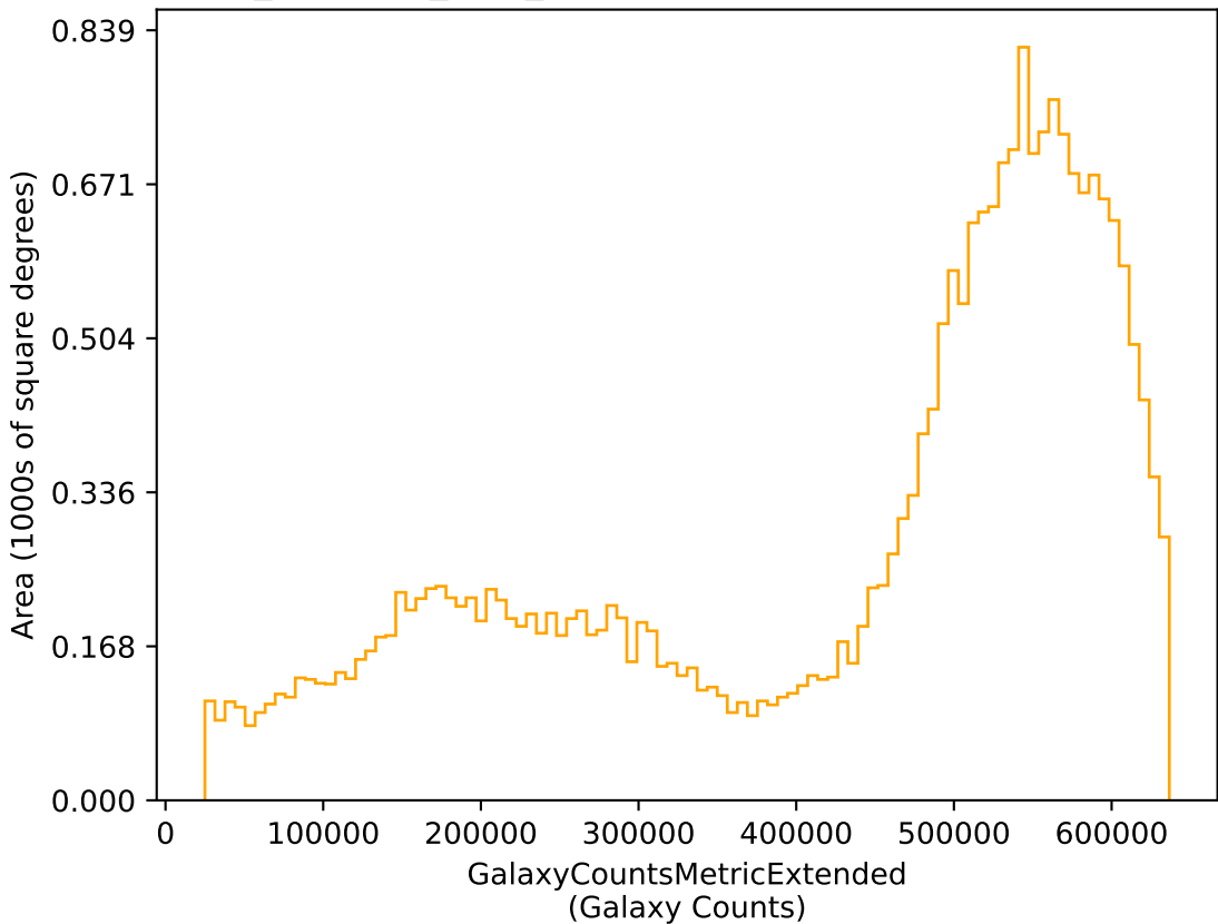
noroll_mjdp365_v3.4_10yrs r: GalaxyCountsMetricExtended
