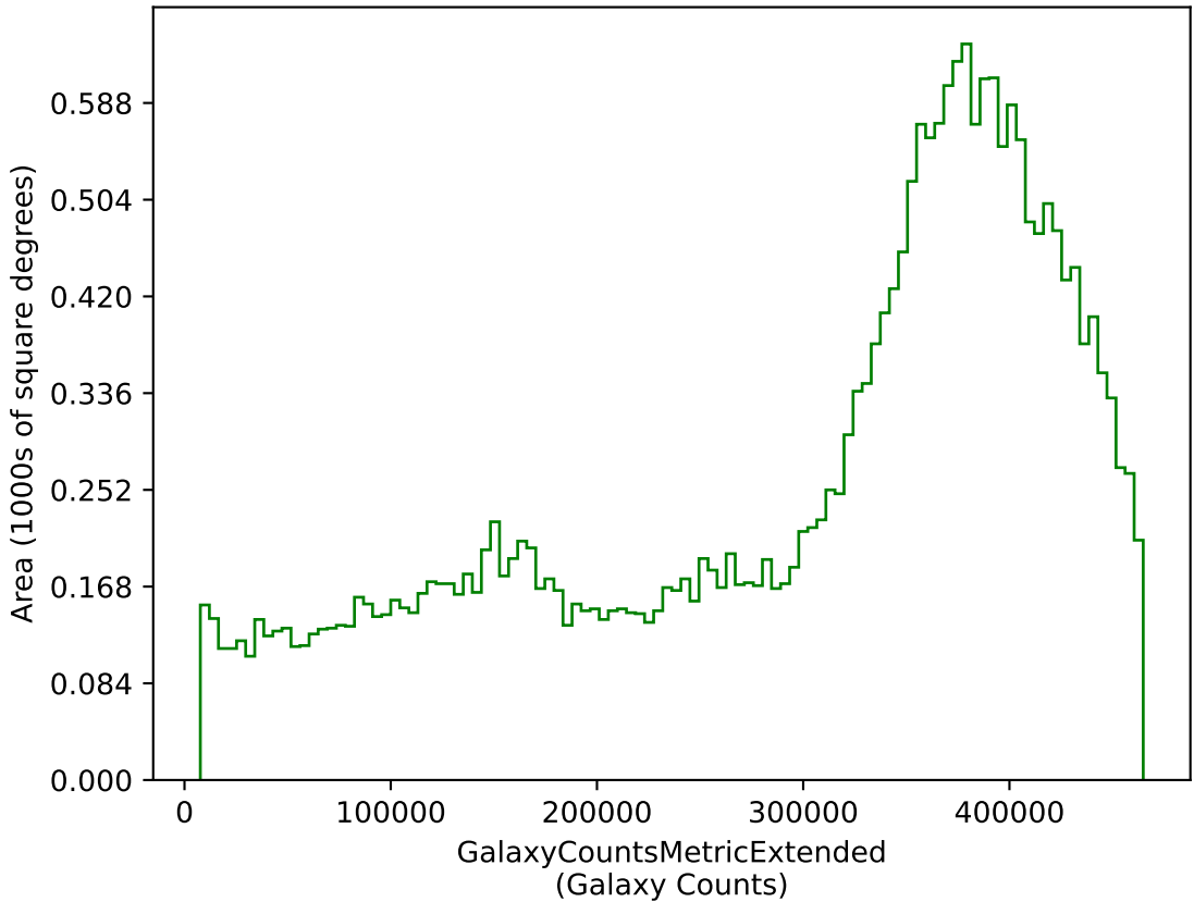
noroll_mjdp365_v3.4_10yrs g: GalaxyCountsMetricExtended
