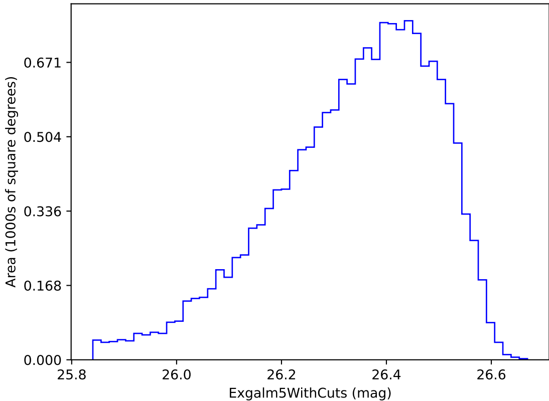
noroll_mjdp365_v3.4_10yrs i band non-DD year 9: ExgalM5WithCuts
