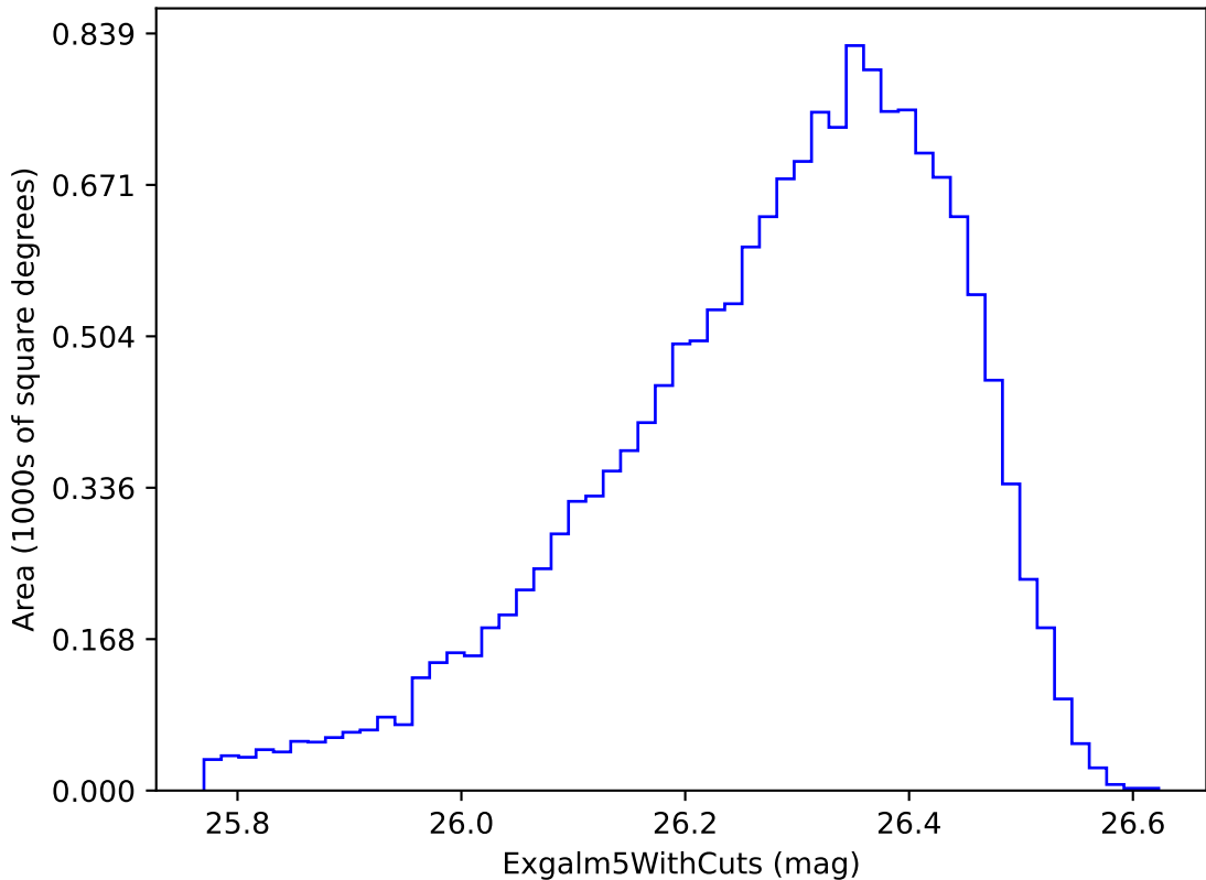
noroll_mjdp365_v3.4_10yrs i band non-DD year 8: ExgalM5WithCuts
