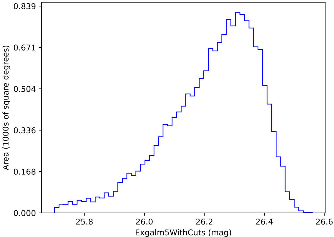
noroll_mjdp365_v3.4_10yrs i band non-DD year 7: ExgalM5WithCuts
